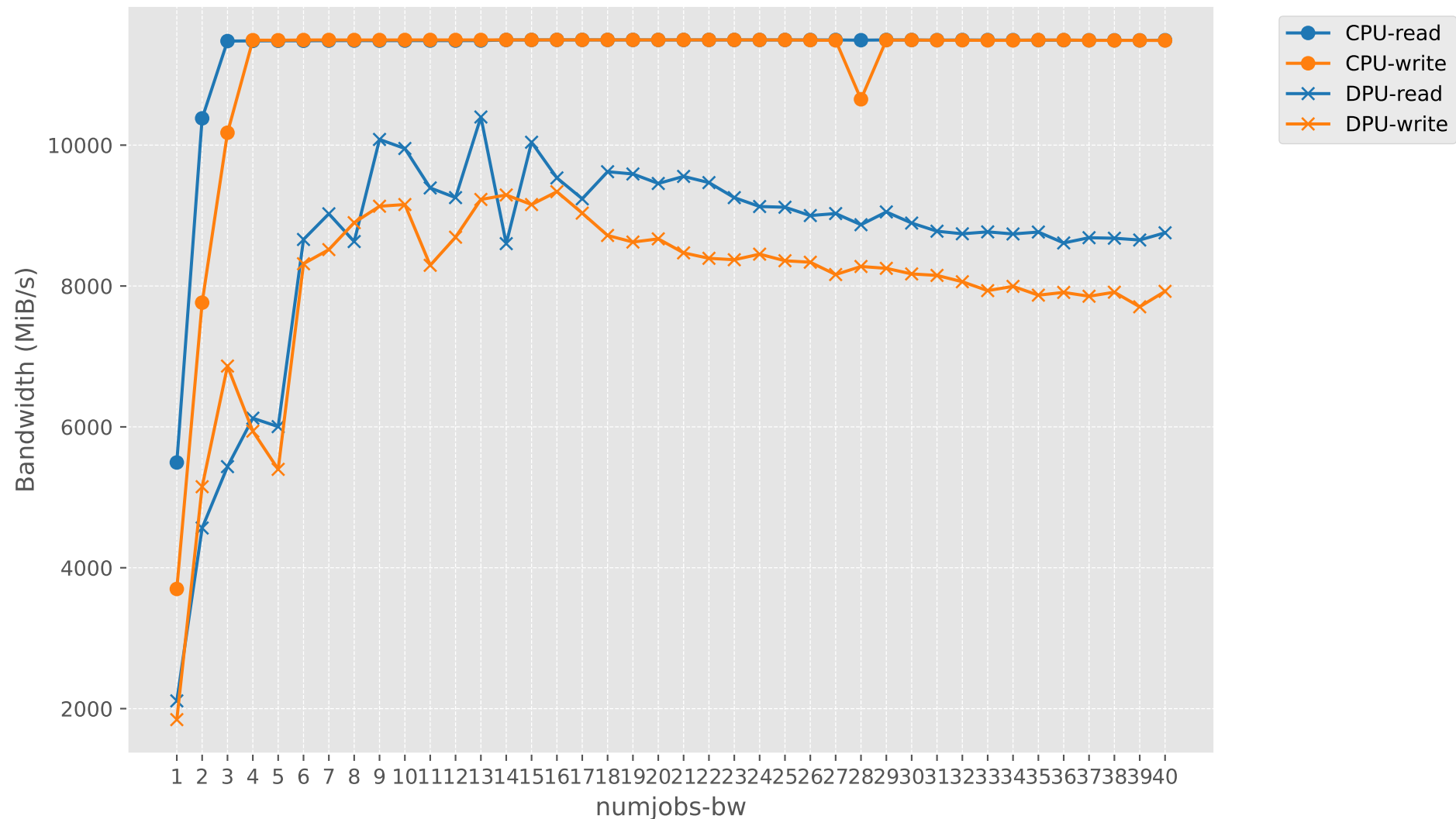
Bandwidth vs numjobs-bw (CPU vs DPU)
